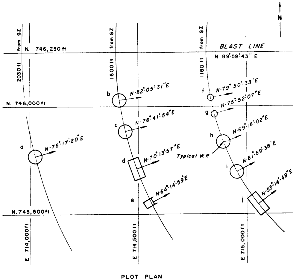
PLOT PLAN
